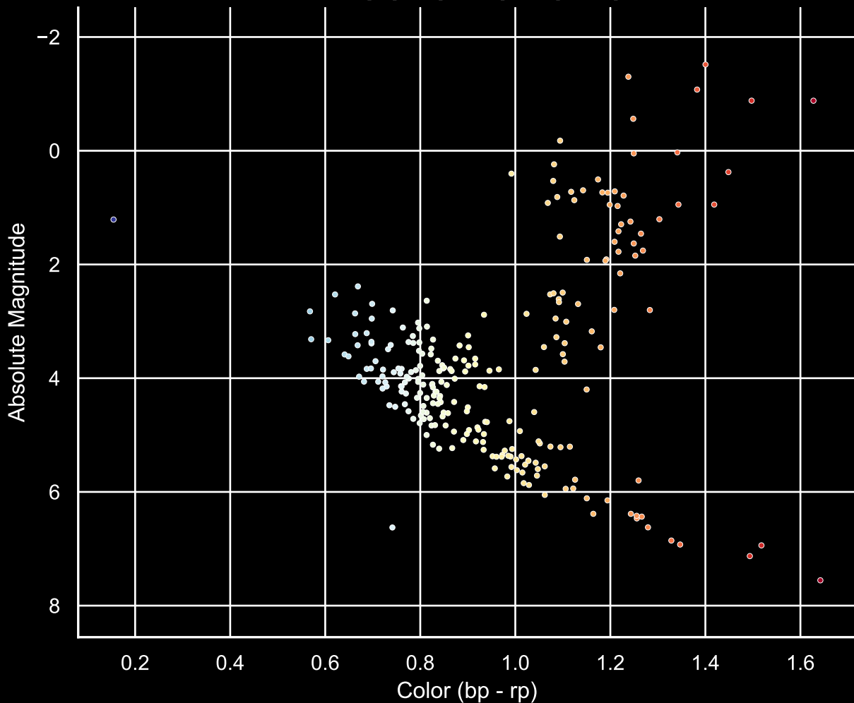
GALAH Hertzprung-Russel Diagram Field [71] Ra [330.06] Dec [-64.58]
