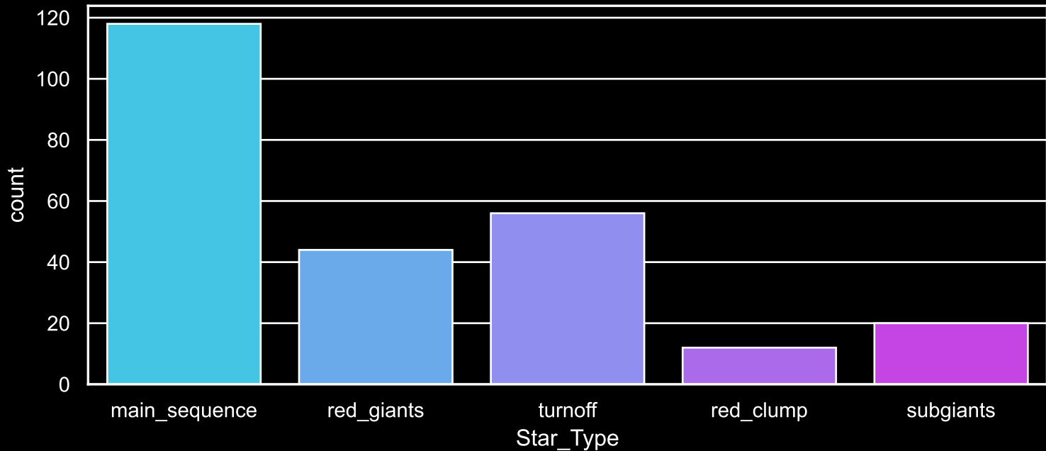
Field [71] Count plot of Star Type
