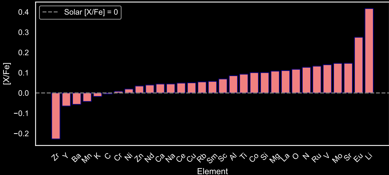
Abundance Pattern for GALAH Star Field [71] (N=250)
