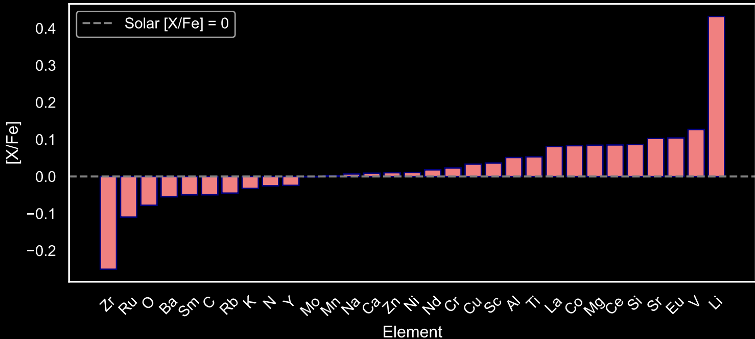
Abundance Pattern for GALAH Main Sequence Stars: Star Field [71] (N=118)
