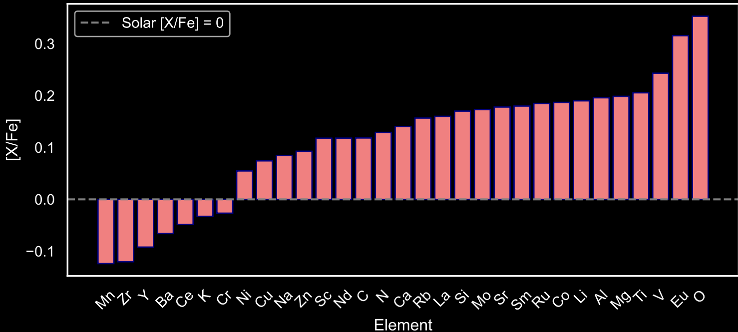
Abundance Pattern for GALAH Red Giants: Star Field [71] (N=56)
